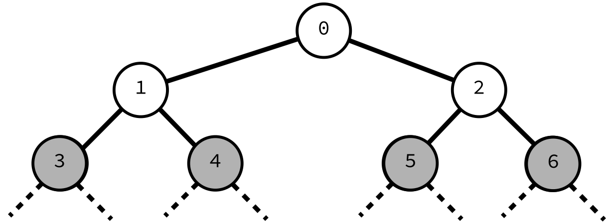
A branch and bound tree. States to explore highlighted in grey.
